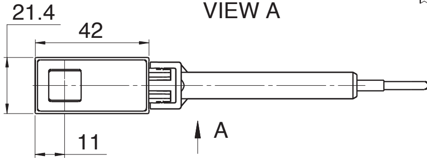
Front View
